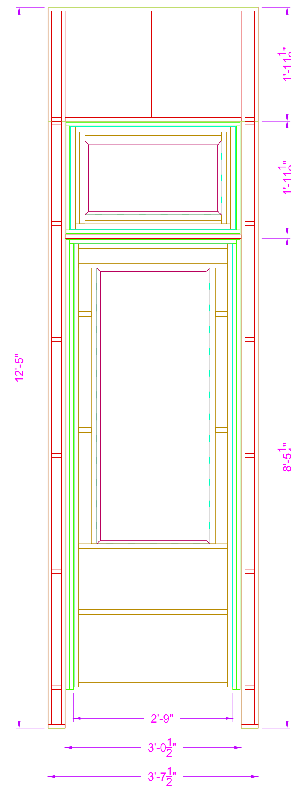
5 SL DOOR WALL - ASSEMBLED FRAMING FRONT VIEW SCALE: 1"=1'-0" QTY: (1)
