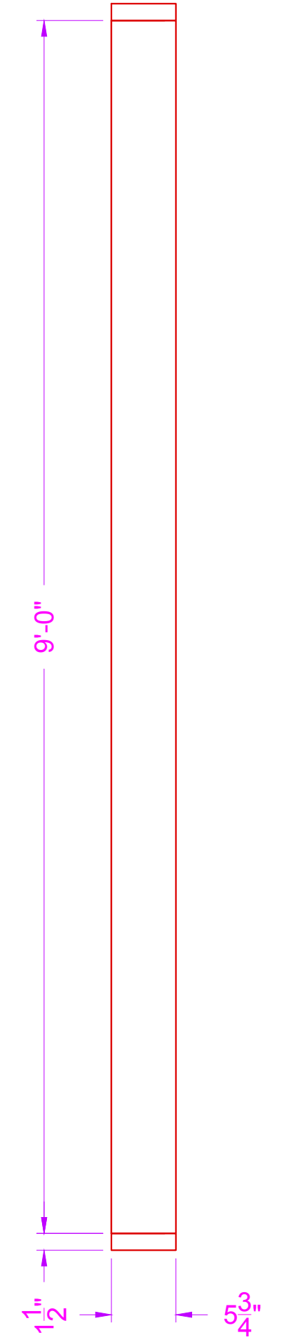
5 WINDOW JAMB (OUTER LAYER) - SIDE VIEW SCALE: 1"=1'-0"
