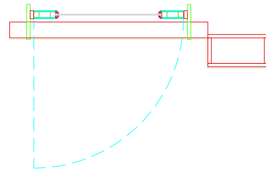
1 SR DOOR WALL - TOP ASSEMBLED VIEW SCALE: 1"=1'-0"
