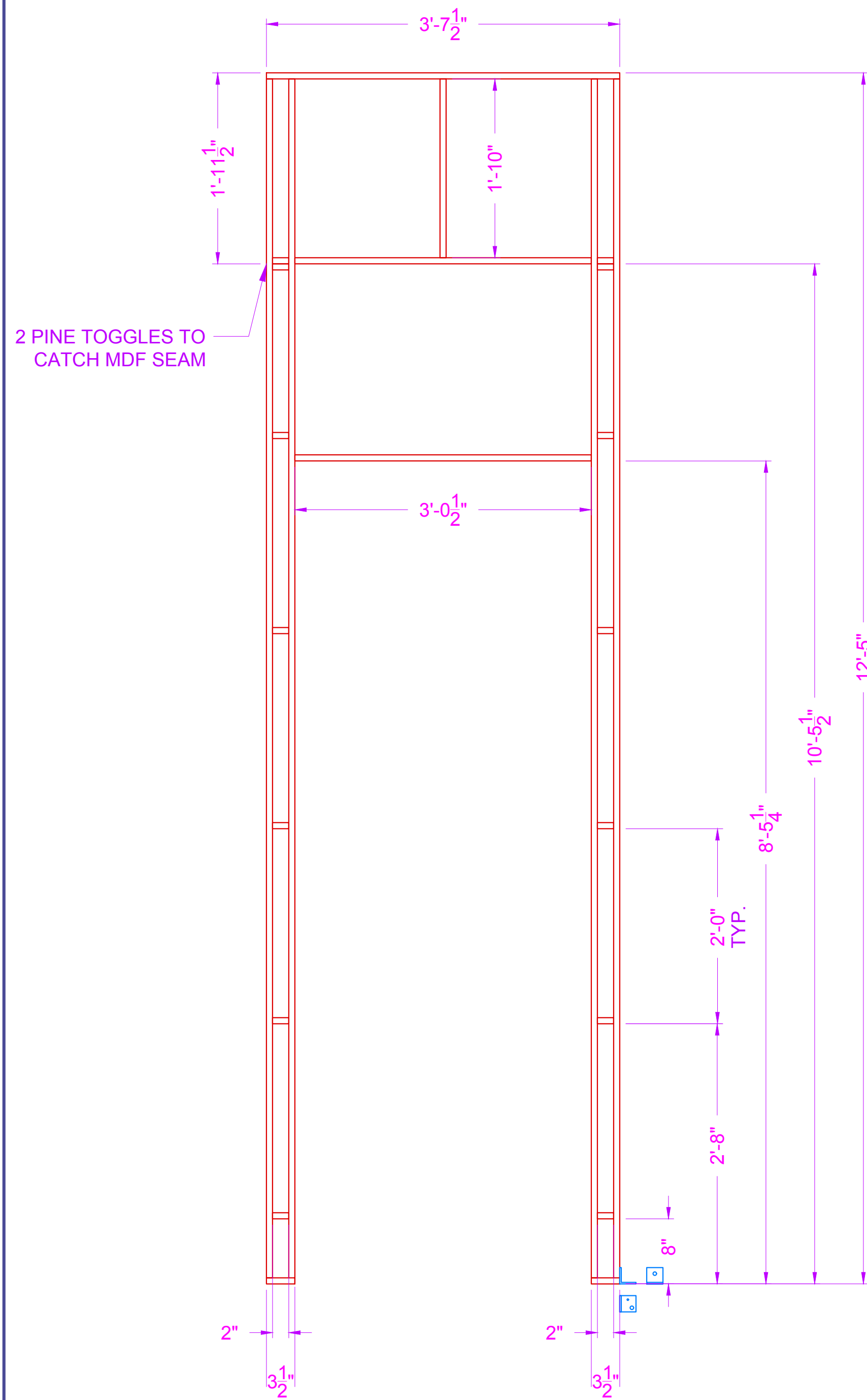
3 SR DOOR WALL - FRONT VIEW - FRAMING SCALE: 1"=1'-0" QTY: (2)
