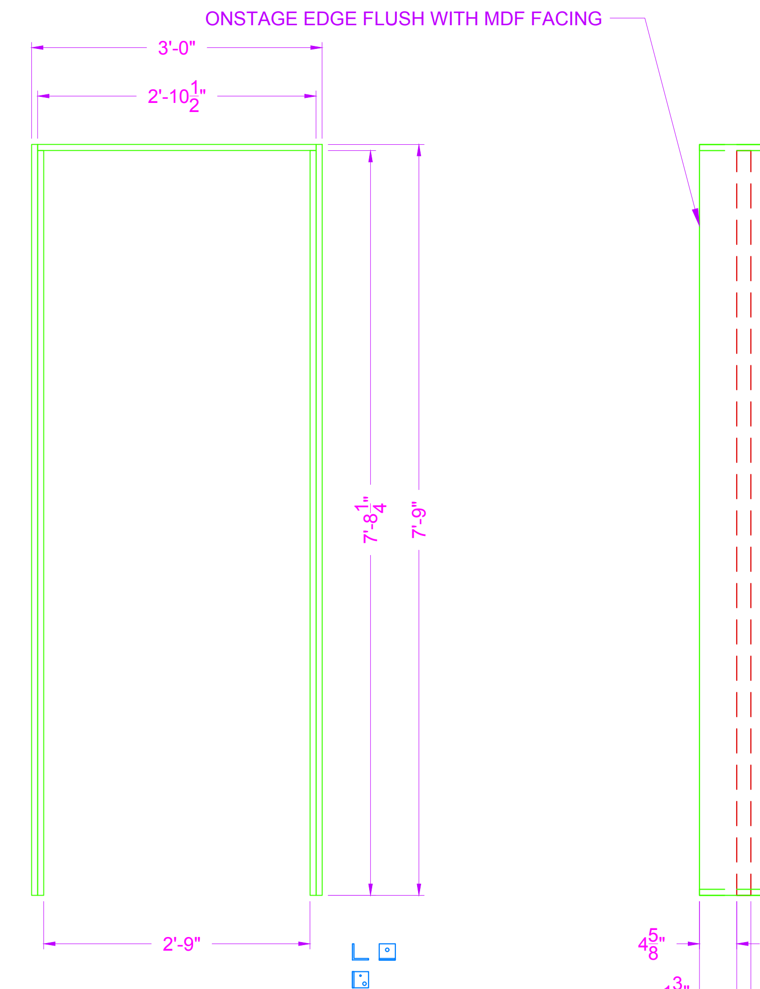
2 DOOR WALL - WINDOW CASING - FRONT VIEW SCALE: 1"=1'-0" QTY: (2)
