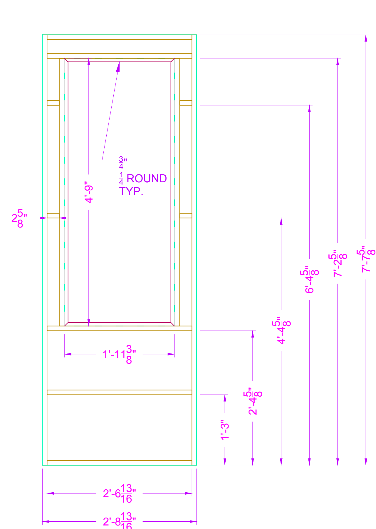
4 DOOR WALL - DOOR - FRONT VIEW SCALE: 1"=1'-0" QTY: TOTAL (2) REVERSE AND REPEAT
