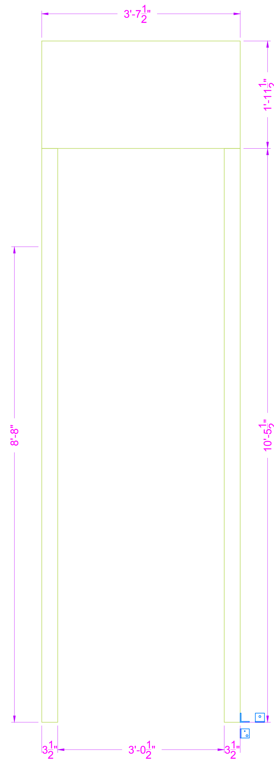
4 SR DOOR WALL - FRONT VIEW - FACING SCALE: 1"=1'-0" QTY: (2)
