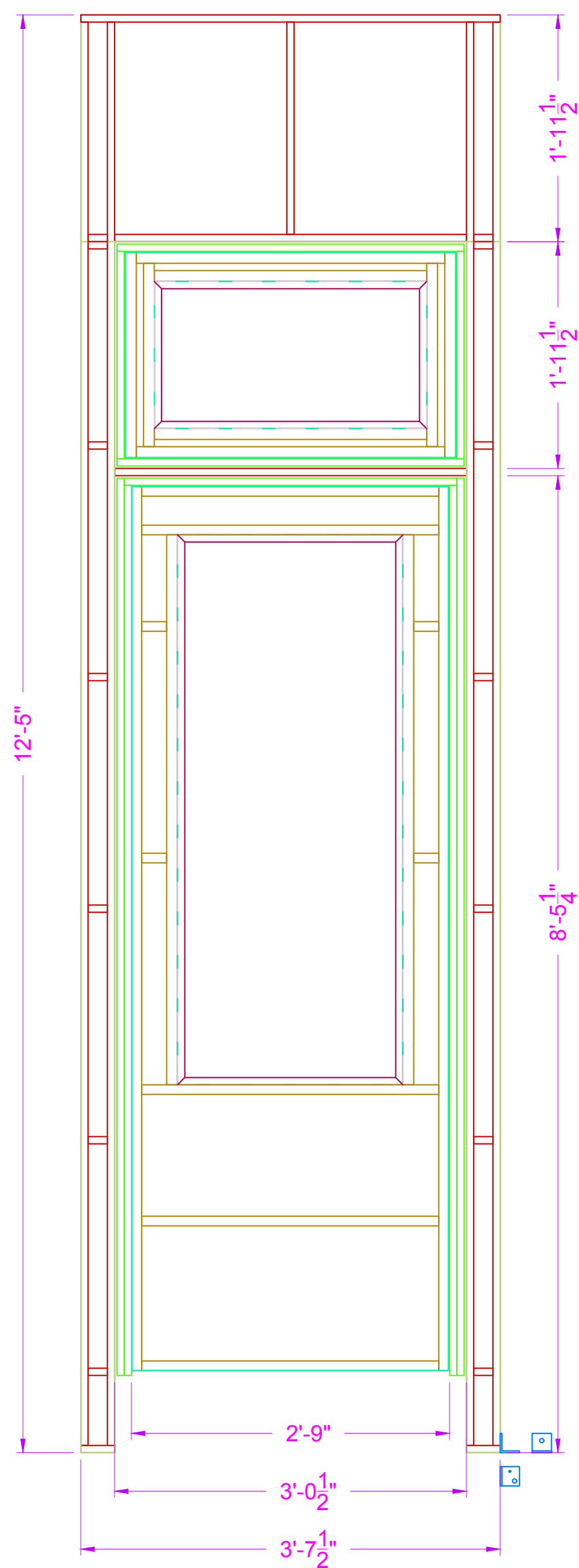
2 SR DOOR WALL - ASSEMBLED FRAMING FRONT VIEW SCALE: 1"=1'-0" QTY: (1)
