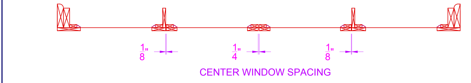
2 WINDOW - SECTION VIEW SCALE: 1"=1'-0"
