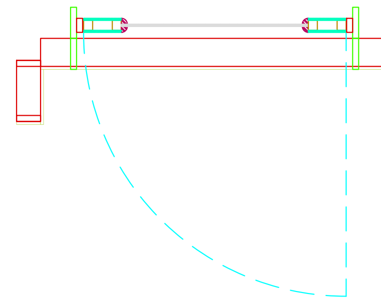
4 SL DOOR WALL - TOP ASSEMBLED VIEW SCALE: 1"=1'-0" QTY: (1)
