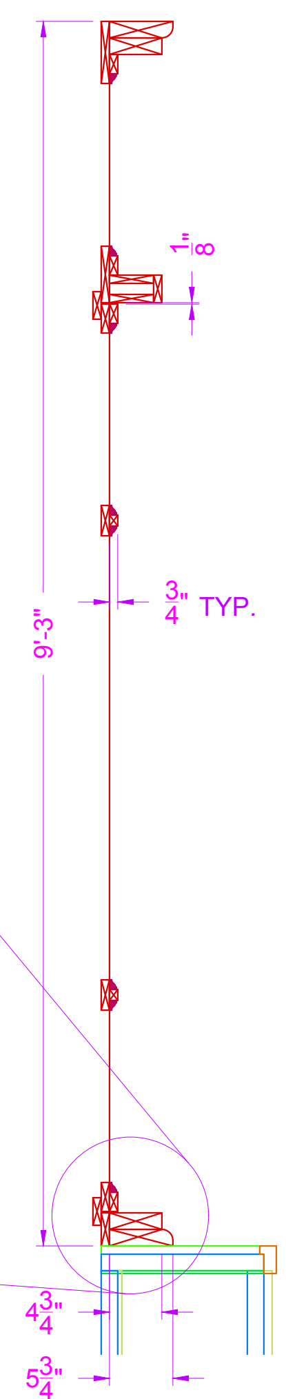
4 WINDOW - SECTION VIEW SCALE: 1"=1'-0"
