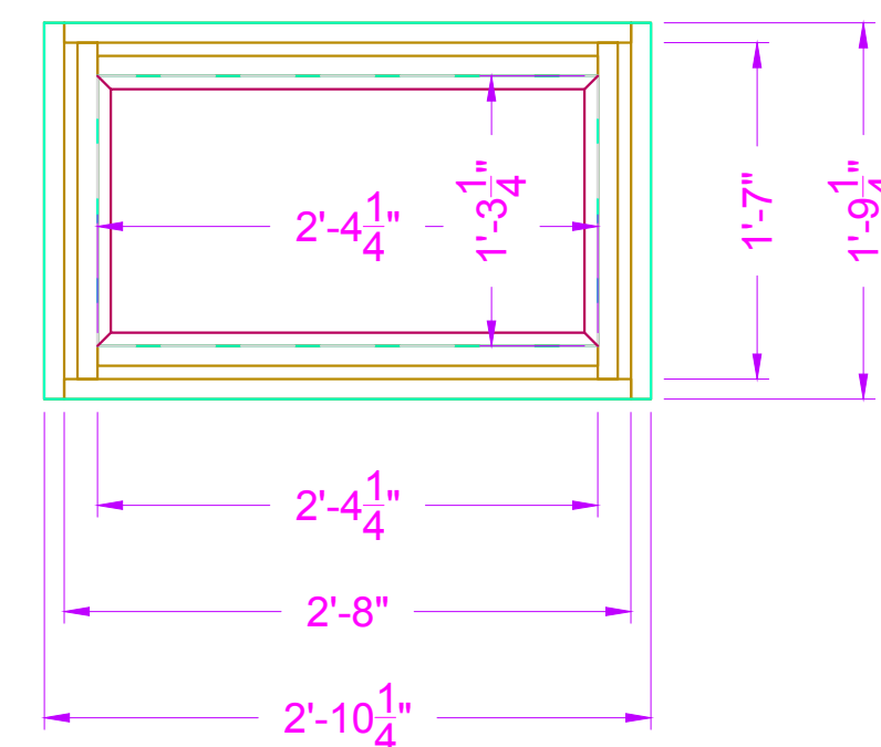
7 DOOR WALL - TRANSOM - FRONT VIEW SCALE: 1"=1'-0" QTY: TOTAL (2)
