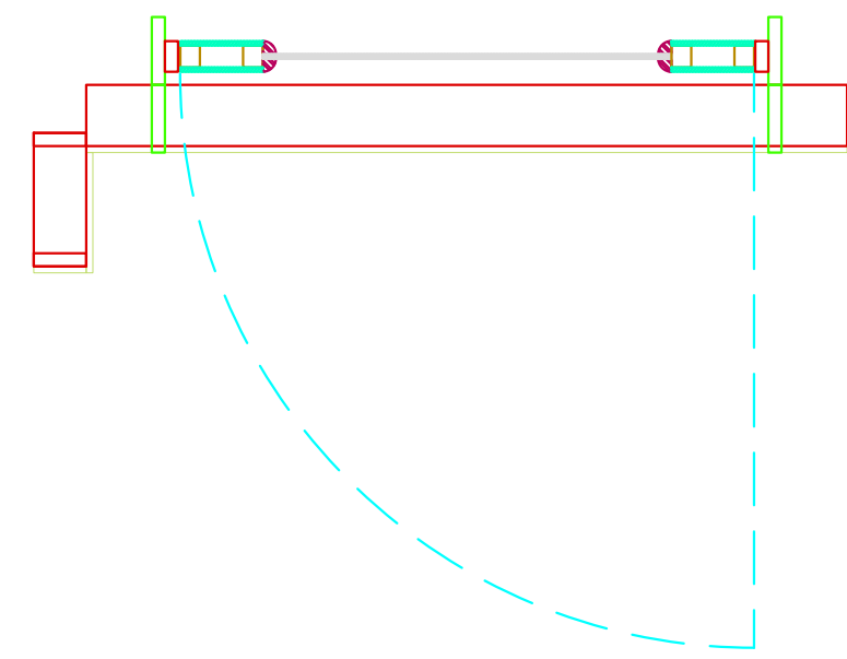
2 SL DOOR WALL - TOP ASSEMBLED VIEW SCALE: 1"=1'-0"
