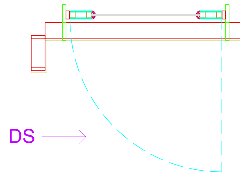
2 SL DOOR WALL - TOP ASSEMBLED VIEW SCALE: 1"=1'-0" QTY: (1)
