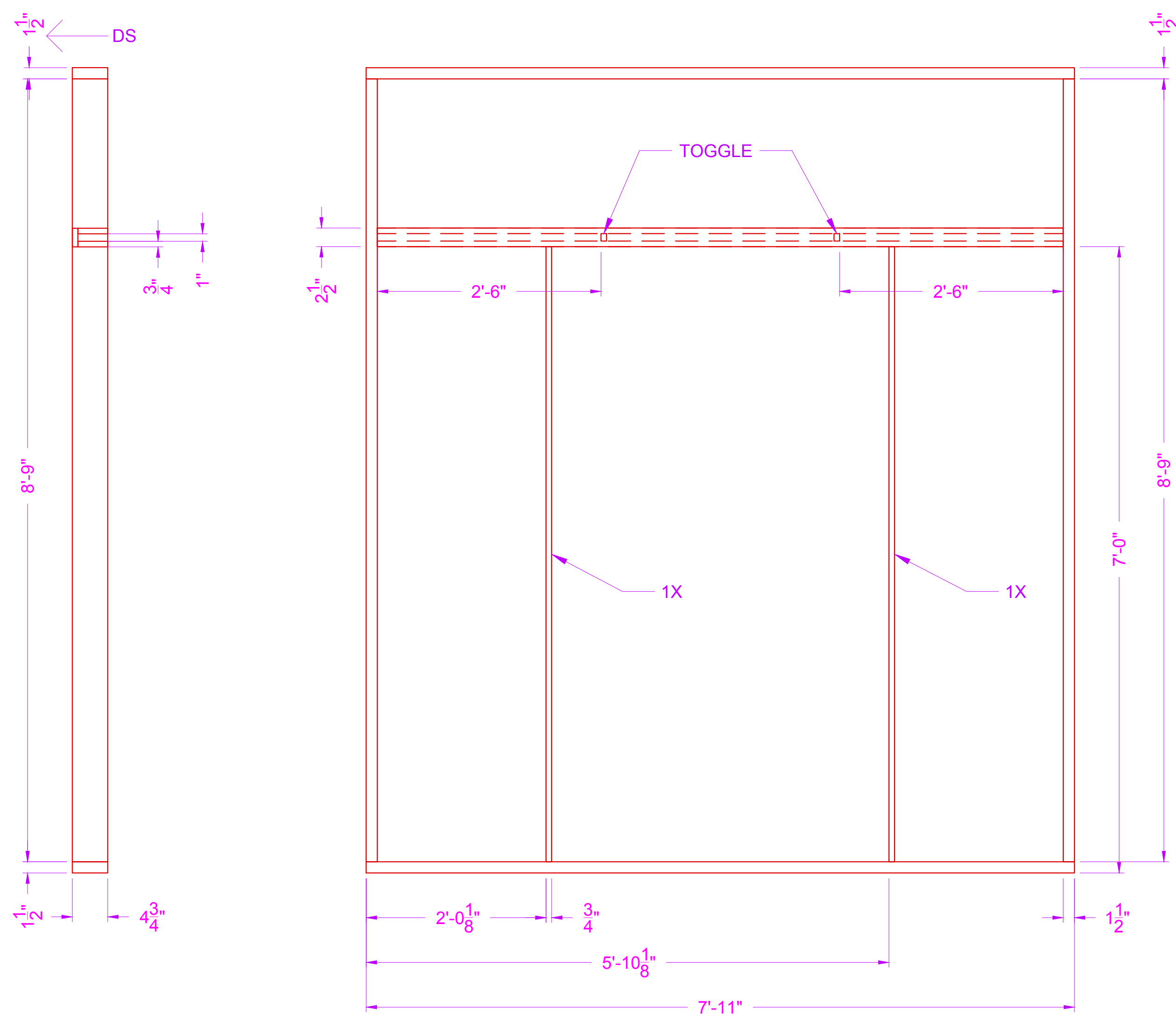
1 WINDOW JAMB (INNER LAYER) - SIDE VIEW SCALE: 1/2"=1'-0" QTY: (1)
