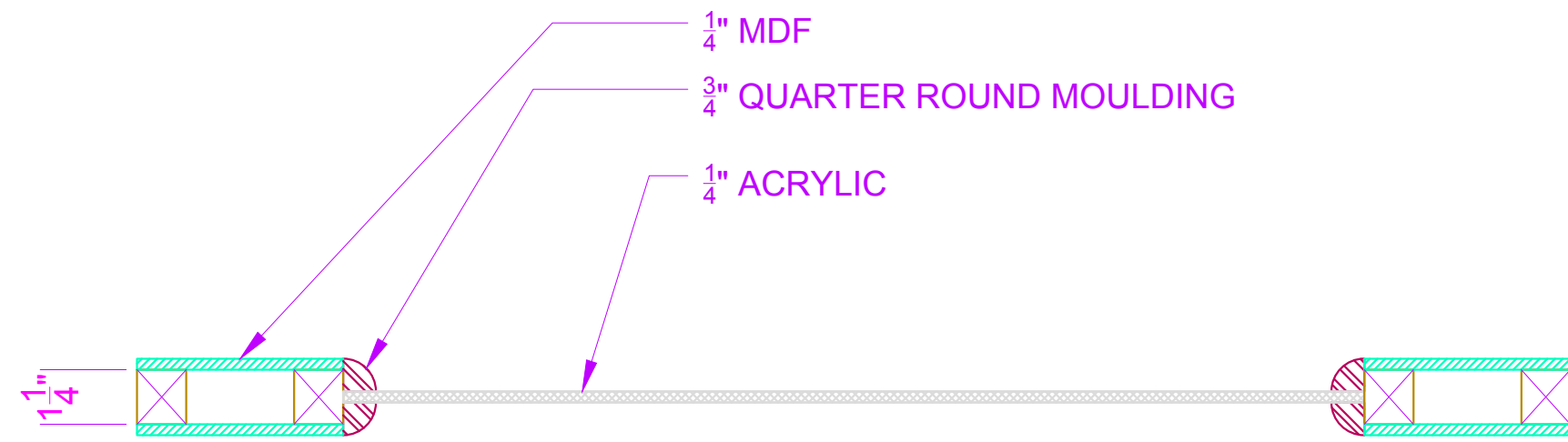
3 DOOR WALL - DOOR - SECTION VIEW SCALE: 3"=1'-0" QTY: (2)
