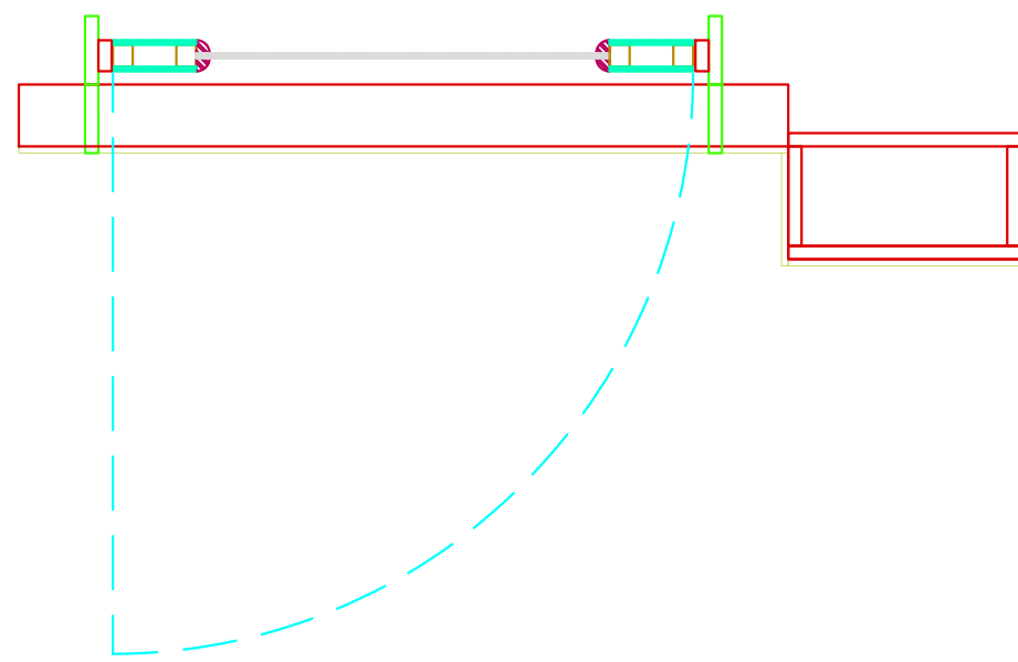
1 SR DOOR WALL - TOP ASSEMBLED VIEW SCALE: 1"=1'-0" QTY: (1)
