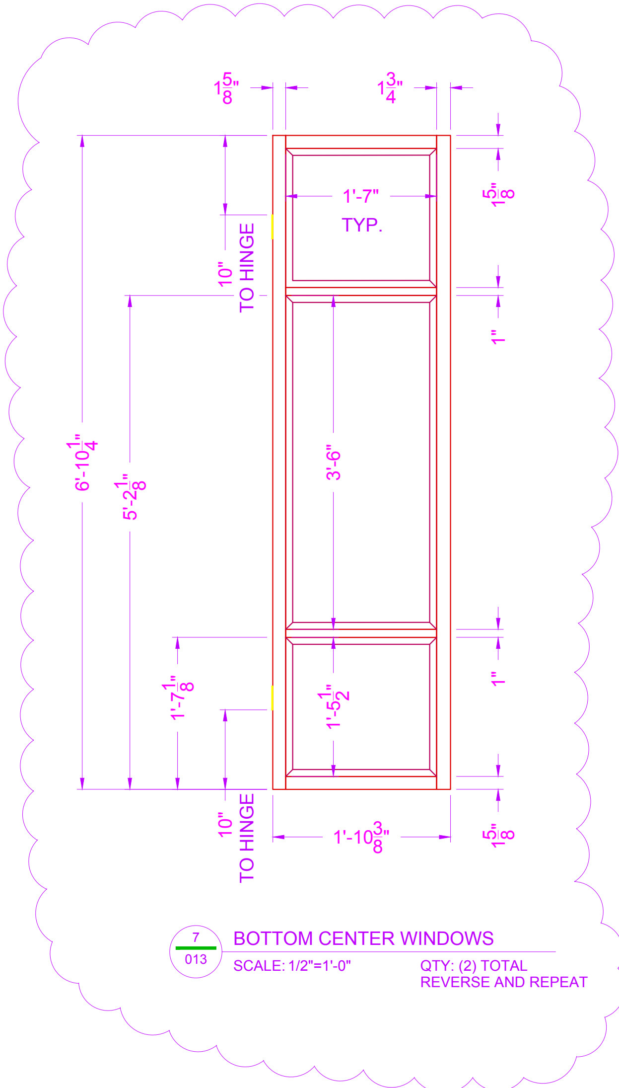
6 BOTTOM CENTER WINDOWS SCALE: 1/2"=1'-0" QTY: (2) TOTAL REVERSE AND REPEAT
