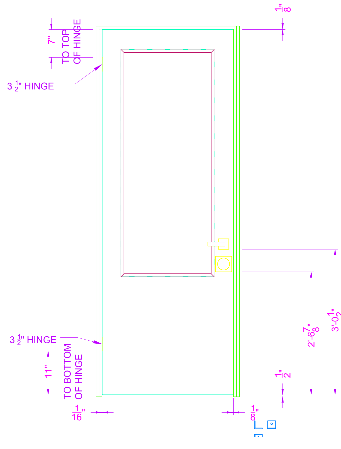
5 DOOR WALL - DOOR HANGING DIMS - FRONT VIEW SCALE: 1"=1'-0" QTY: TOTAL (2) REVERSE AND REPEAT
