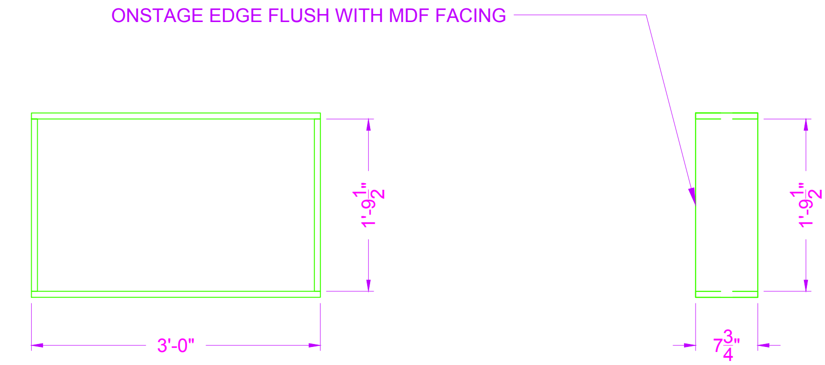
2 DOOR WALL - WINDOW CASING - FRONT VIEW SCALE: 1"=1'-0" QTY: (2)
