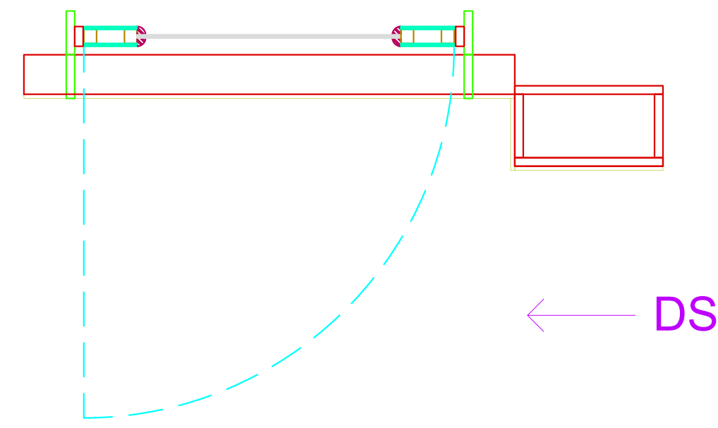
1 SR DOOR WALL - TOP ASSEMBLED VIEW SCALE: 1"=1'-0" QTY: (1)
